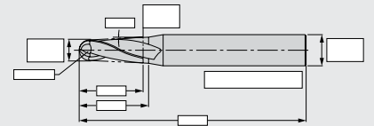
TAPER BALLNOSE
